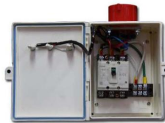
Breaker 15, 30Amp 220V. 50Hz. 1 Phase
